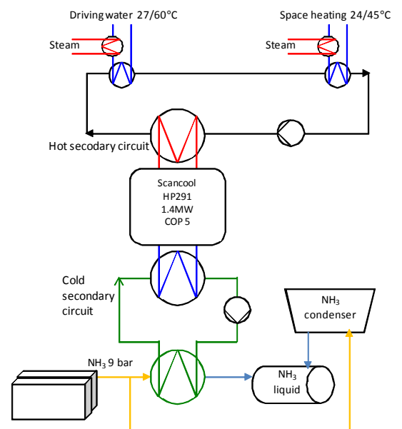
A conceptual view of the heat pump system.
